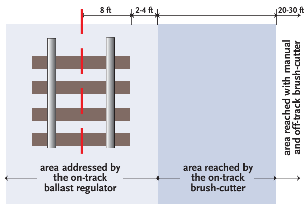
On-track brush-cutter.
