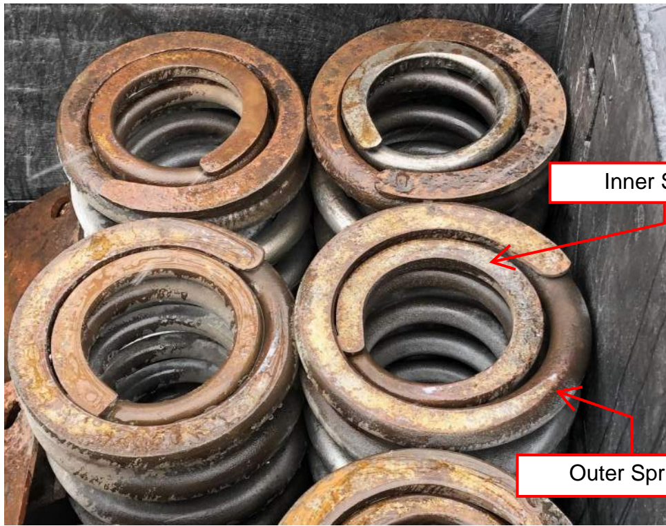
Bolster Springs (Bigger Springs), Four per Truck Unit
