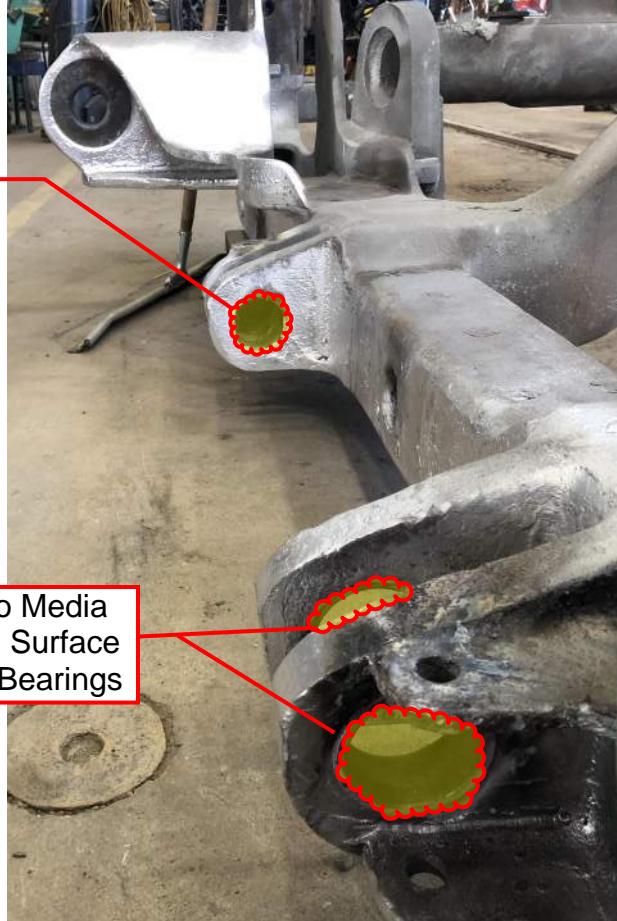
Truck Frame, 1 per Truck Unit
