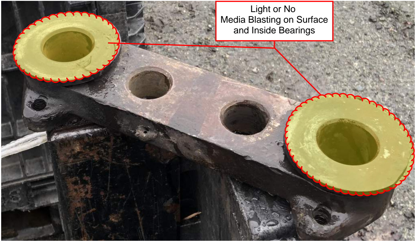
Brake Arm Tie Bar, 8 per Truck Unit
