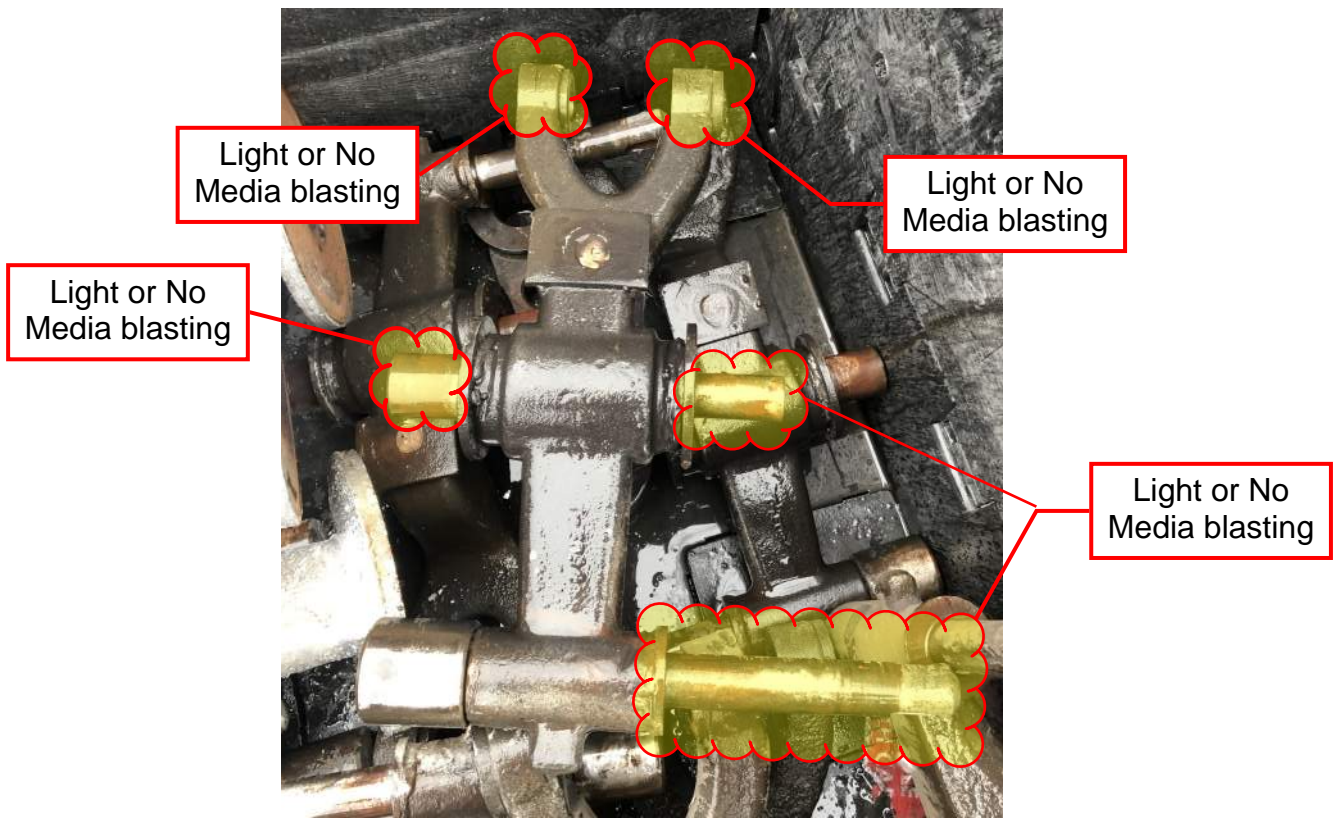
Brake Arm, Eight per Truck Unit
