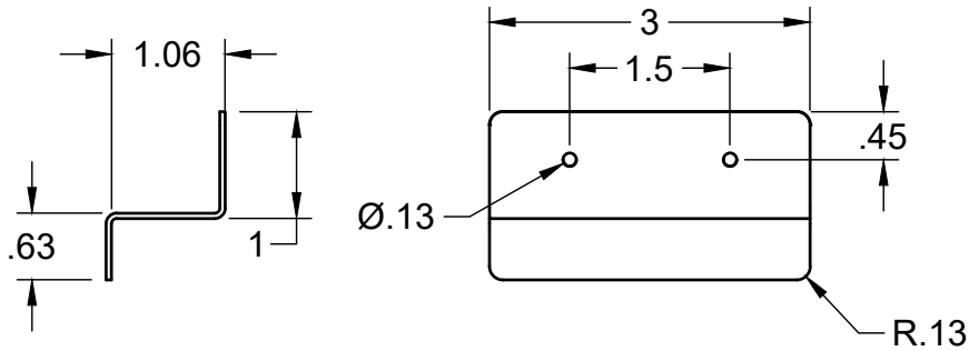
ARRC DINING SEAT BRACKET 'A' PN: ARR-XXX-0001 MATERIAL: 18GA GALVANNEALED STEEL
